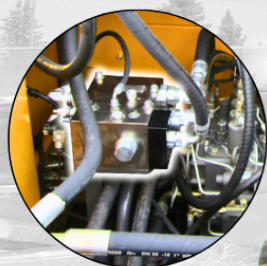
Priority Valve
